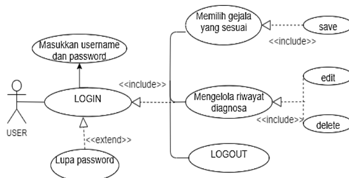
Gambar 3. Usecase diagram user
