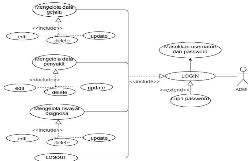
Gambar 2. Usecase diagram admin
