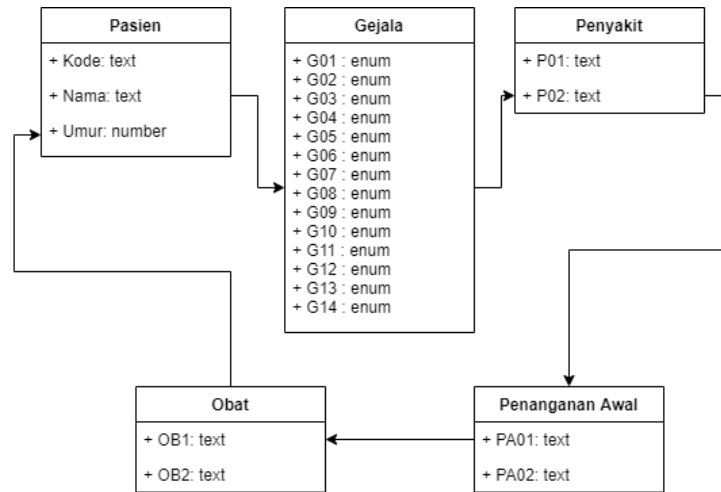
Gambar 6. Entitas rancangan basis data
