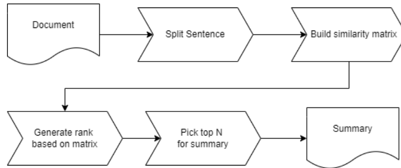
Figure 5. The Extractive Text Summarization Process
