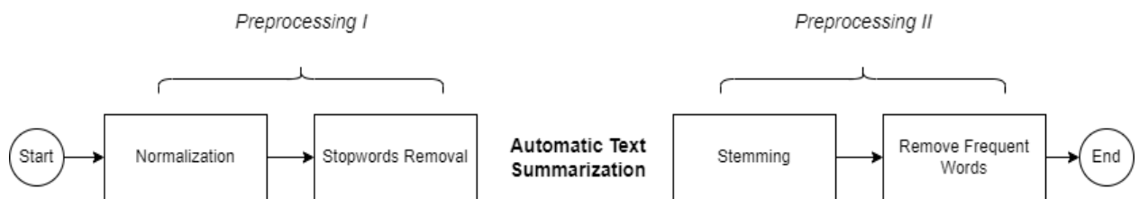
Figure 3. Preprocessing Stages
