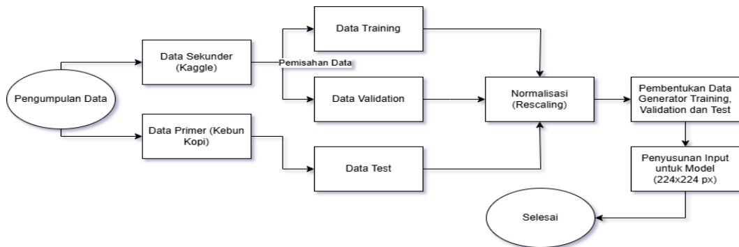
Gambar 2. Alur Data Preparatorion
