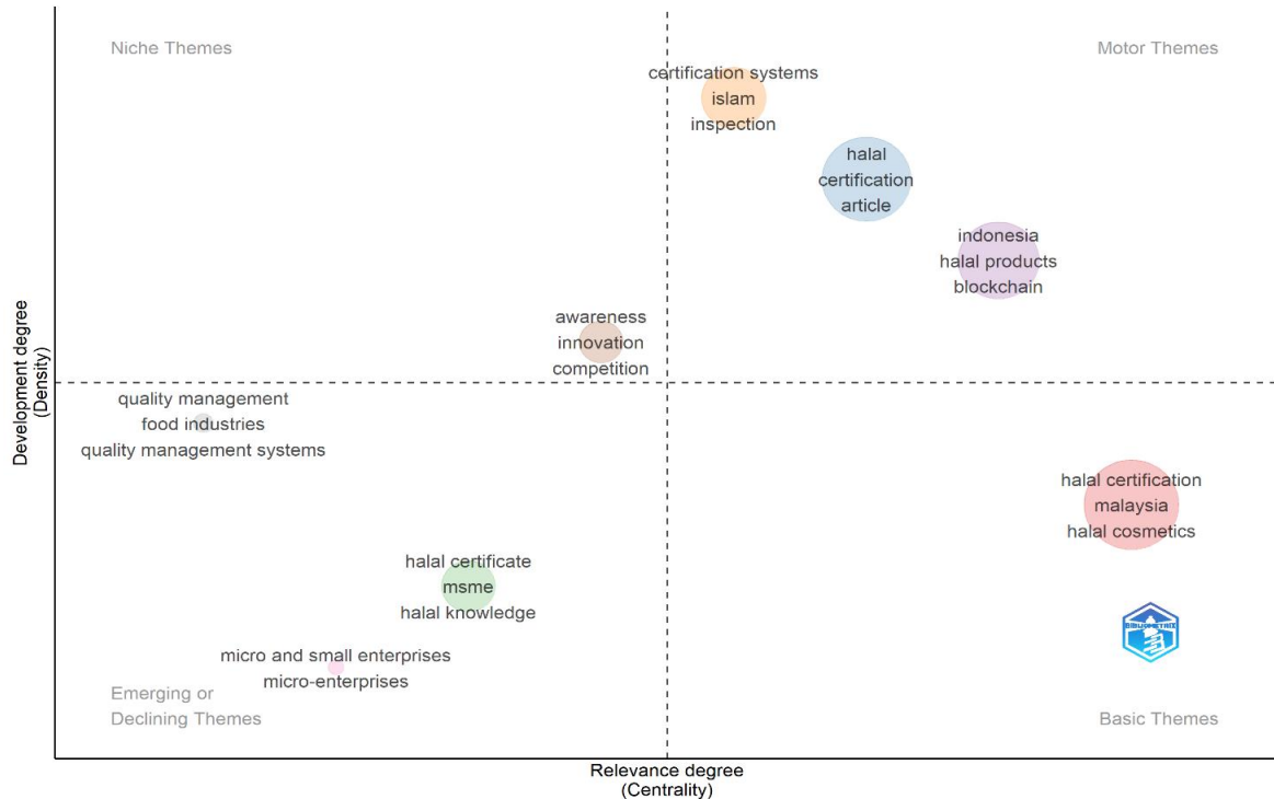
Gambar 5. Thematic Map Penelitian Sertifikasi Halal
